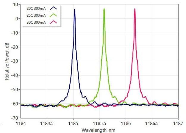
Optical Spectra vs Temperature (res. 10pm)
