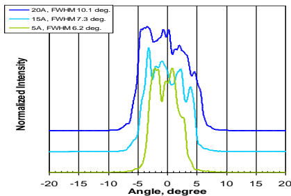
CW Slow Axis Far Field
