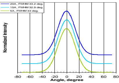
CW Fast Axis Far Field
