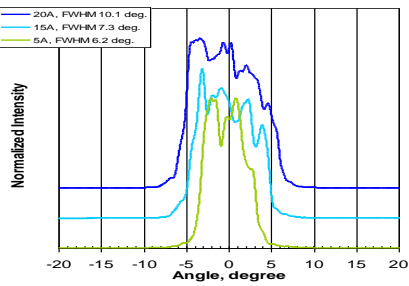
CW Slow Axis Far Field
