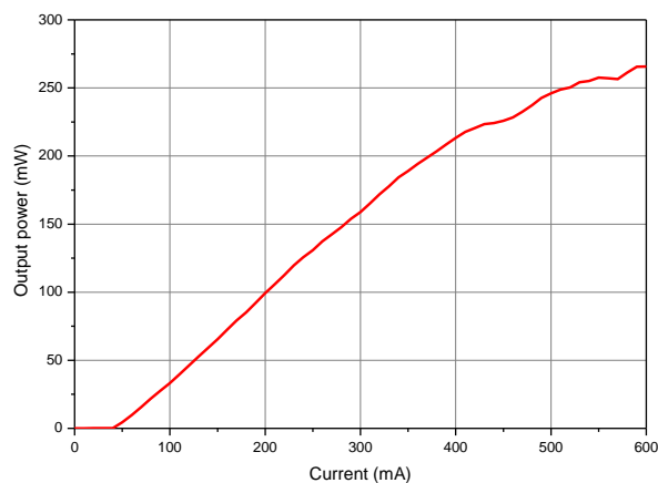
Output power @ 1090 nm
