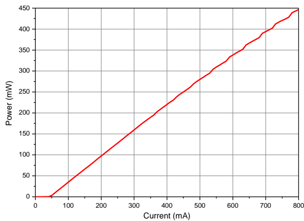
Output power @ 1110nm
