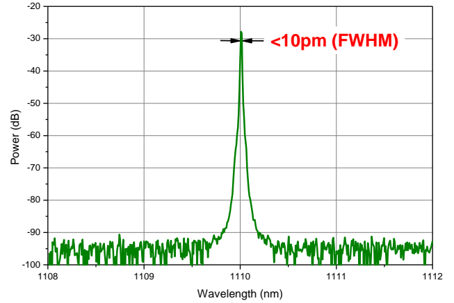
Optical spectrum @ 600mA (res. 10 pm)
