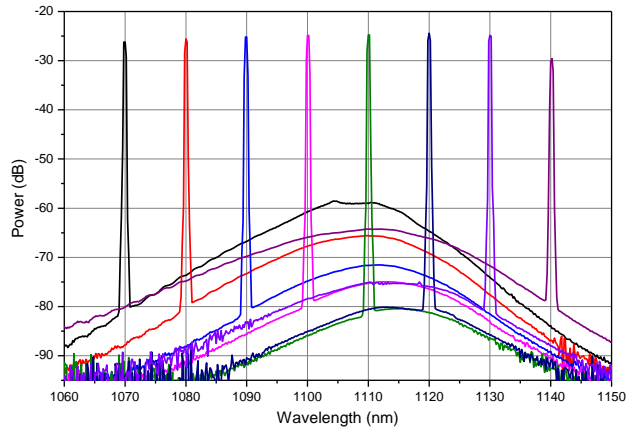
Optical spectra @ 600mA (res. 0.5 nm)
