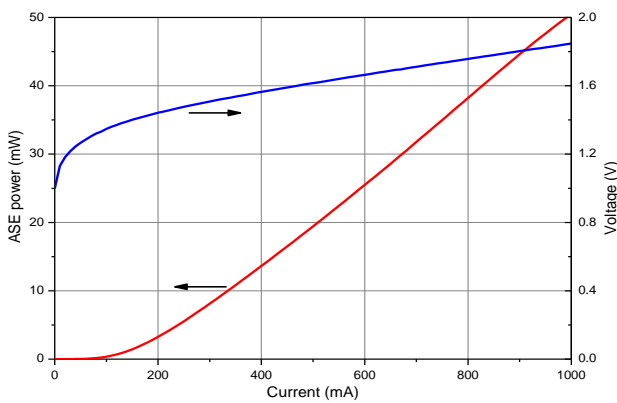
Light-Current-Voltage Characteristics
