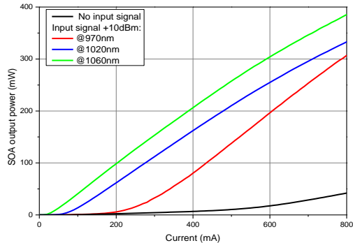
Output power at different input signals
