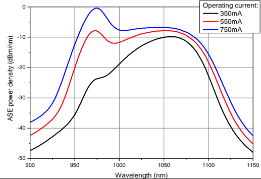
ASE Spectra (no input signal)
