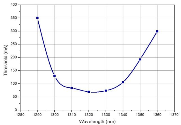
Threshold current
